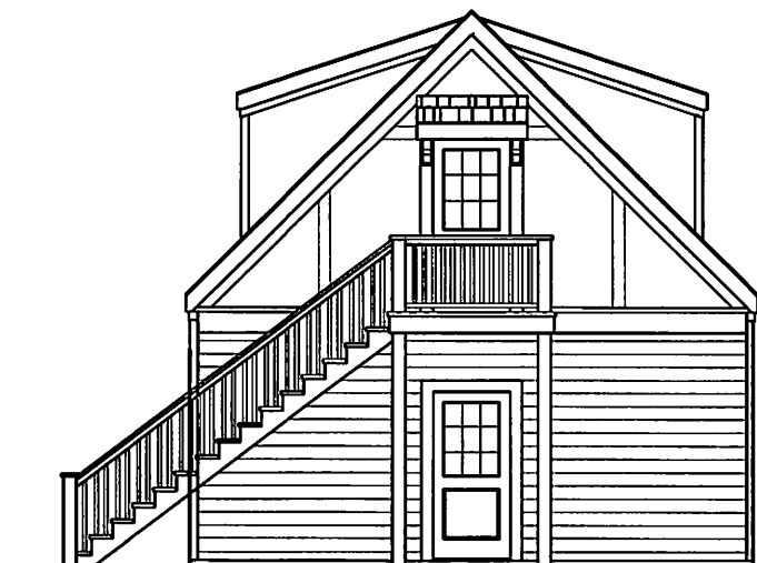
1361 MIDDLESEX AVE. GARAGE RIGHT ELEVATION
