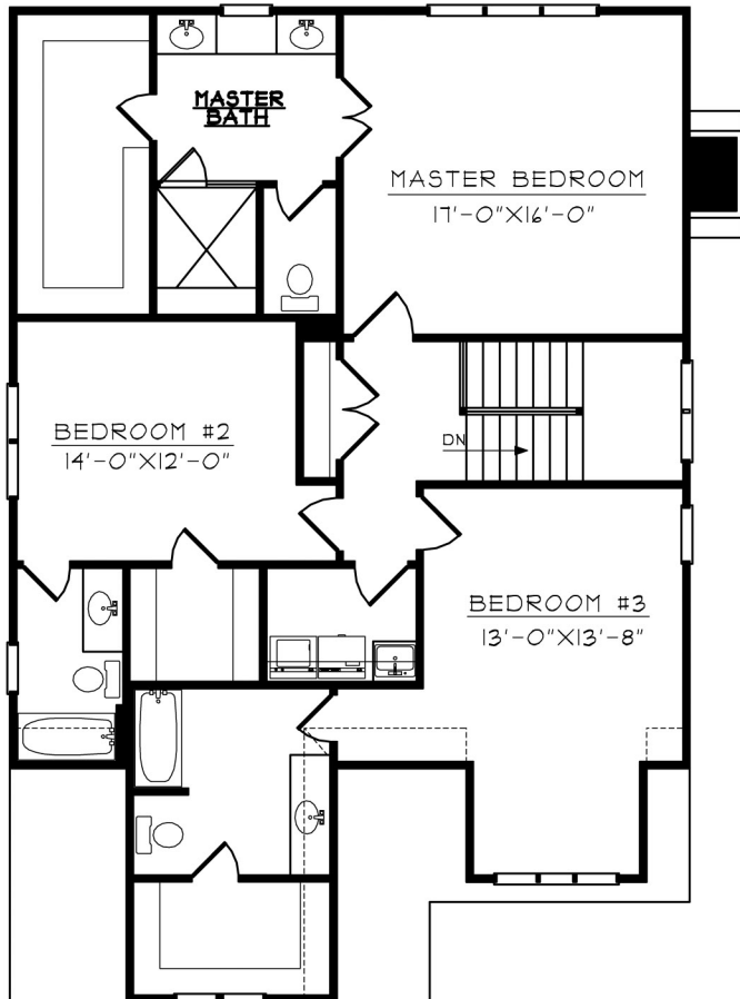
439 PENSDALE RD. SECOND FLOOR PLAN
