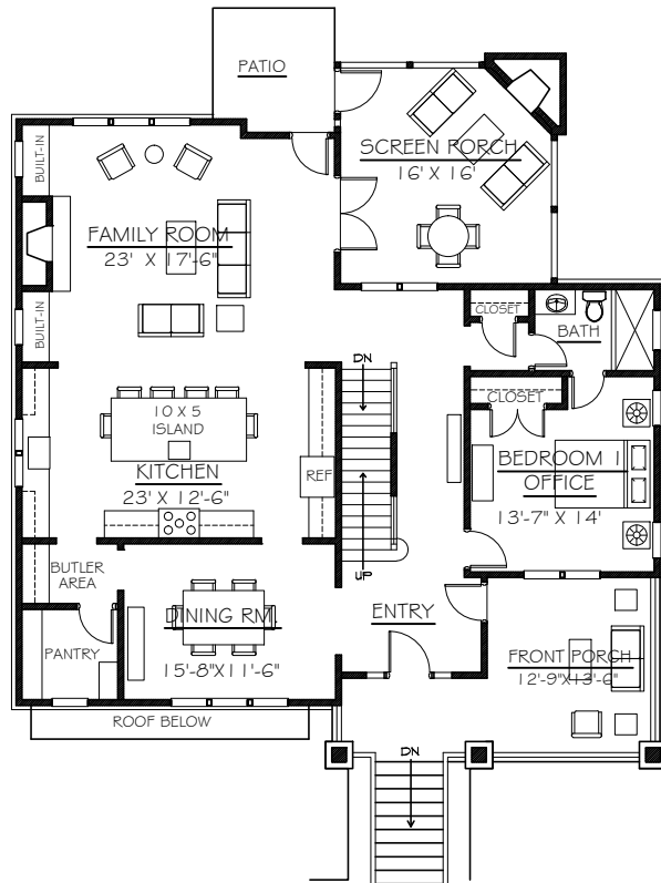
FIRST FLOOR PLAN 1,619 SF
