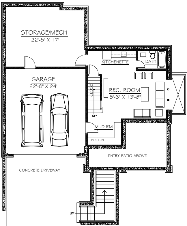
LOWER LEVEL & GARAGE LOWER LEVEL FINISHED AREA: 604 SF
