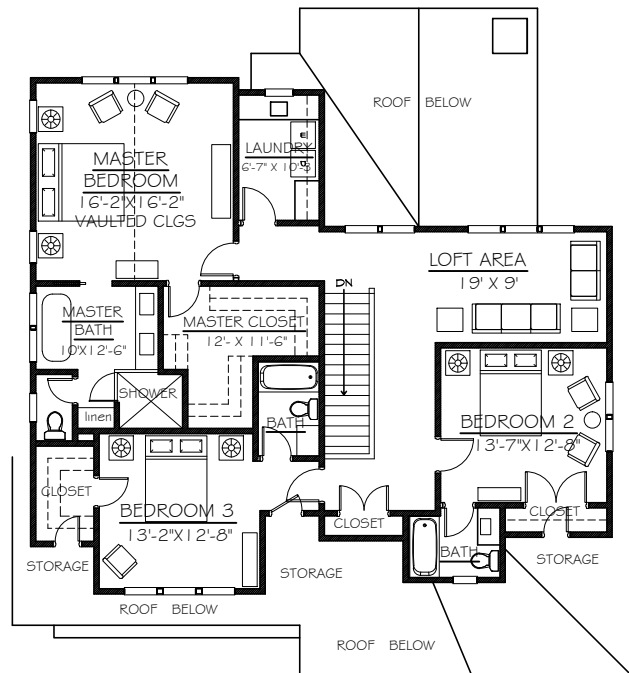
SECOND FLOOR PLAN 1,584 SF
