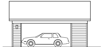
CARPOT SIDE ELEV.
